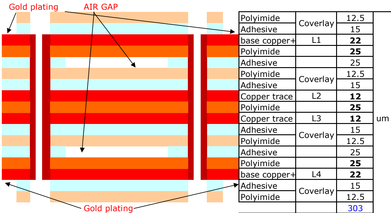
Best Technology 4L FPC (Unbonded) Stack Up (Option B) 1L+2L+1L FPC, suitable for LW/LS <=4mil
